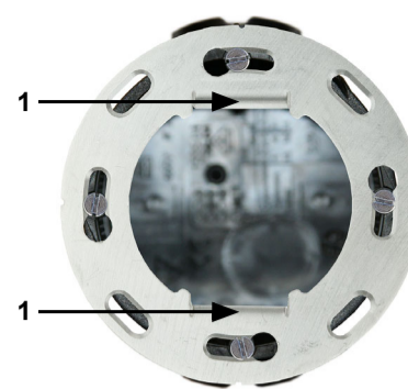
Fig. 6 Connector socket with Ø 60 mm, 42 mm deep. 1 Support ring, screwed to the socket 2 Springs hold the device firmly on the support ring
