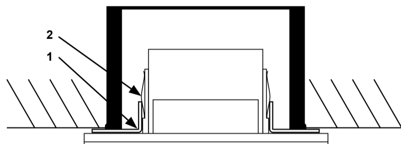
Fig. 6 Connector socket with Ø 60 mm, 42 mm deep. 1 Support ring, screwed to the socket 2 Springs hold the device firmly on the support ring
