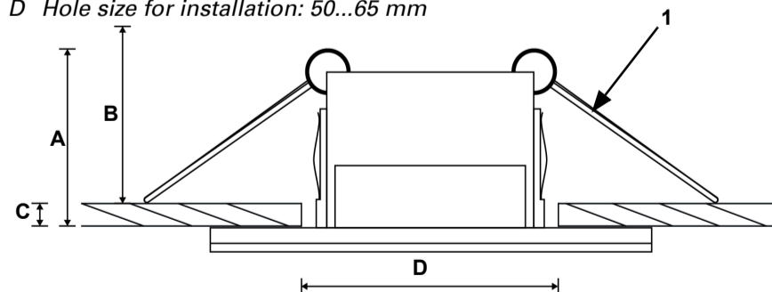
Fig. 4 1 Clamps for installation in false ceiling A Height in wall (built-in): approx. 31 mm B Space behind the false ceiling, necessary for insertion (clear dimension): approx. 31 mm C Maximum wall thickness: 20 mm D Hole size for installation: 50...65 mm
