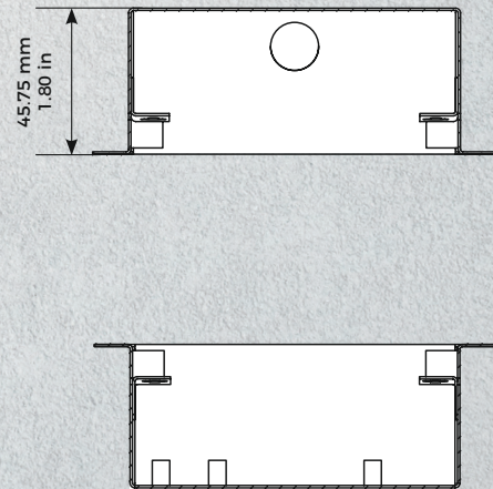
Mounting housing
